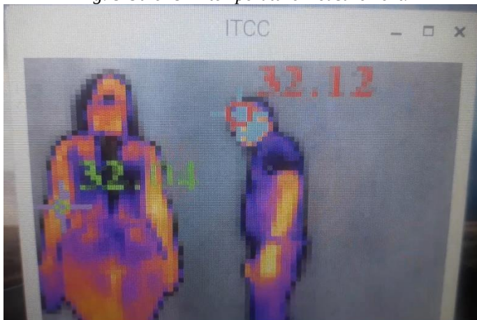
Fig. 9 Two-target skin temperature measurement.
