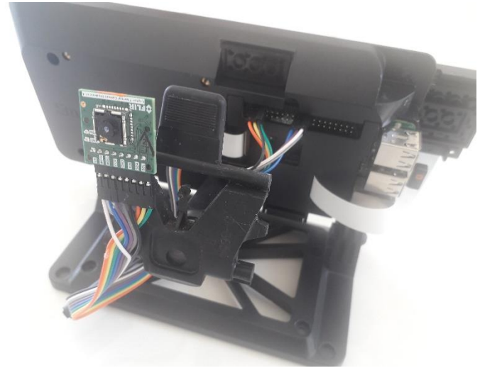
Fig. 6 Lepton + RPi + 7" Touchscreen + SmartiPi Touch.
