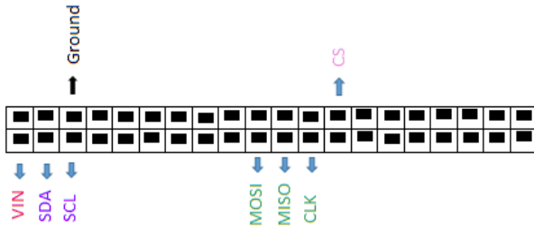
Fig. 3 Lepton & RPi Connection.
