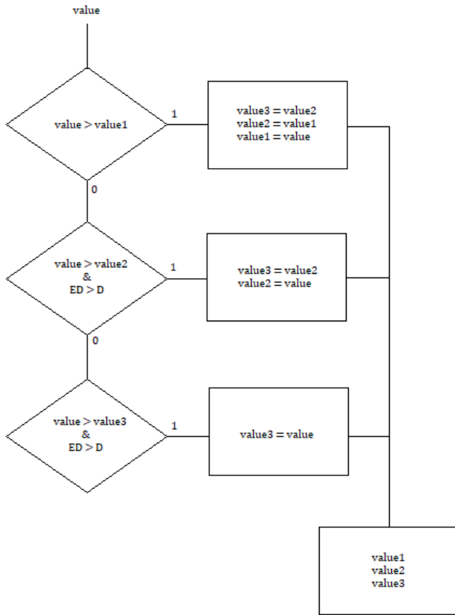
Fig. 5 Getting 3 hottest and separated temperatures.
